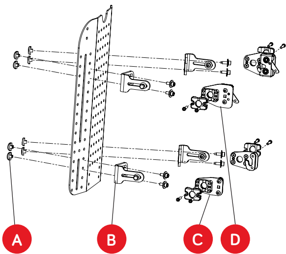
HEAVY DUTY QUAD MOUNT OVERVIEW
