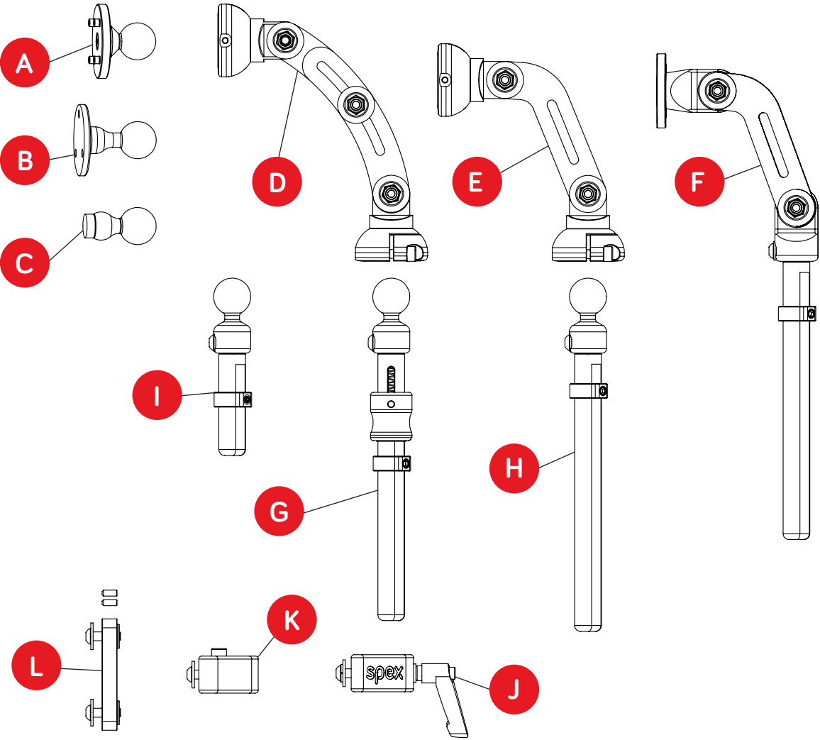
STYLO HEAD SUPPORT
