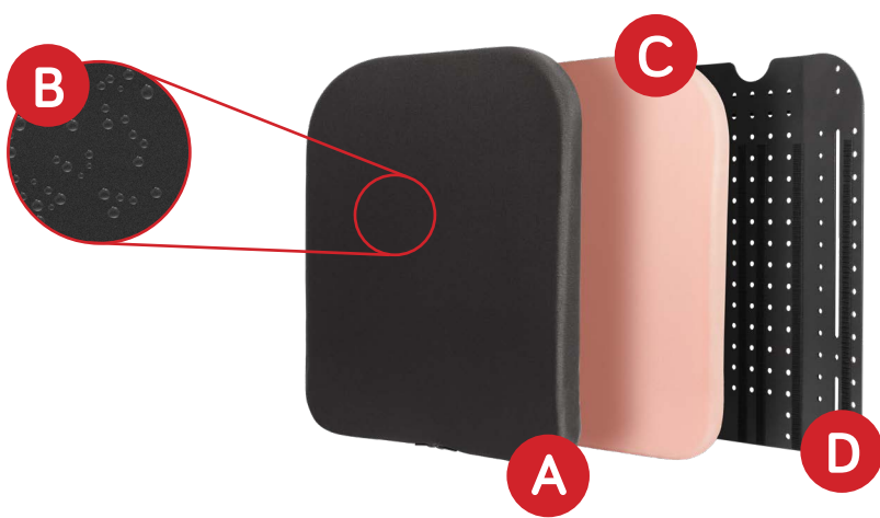
VIGOUR BACK SUPPORT - EXPLODED
