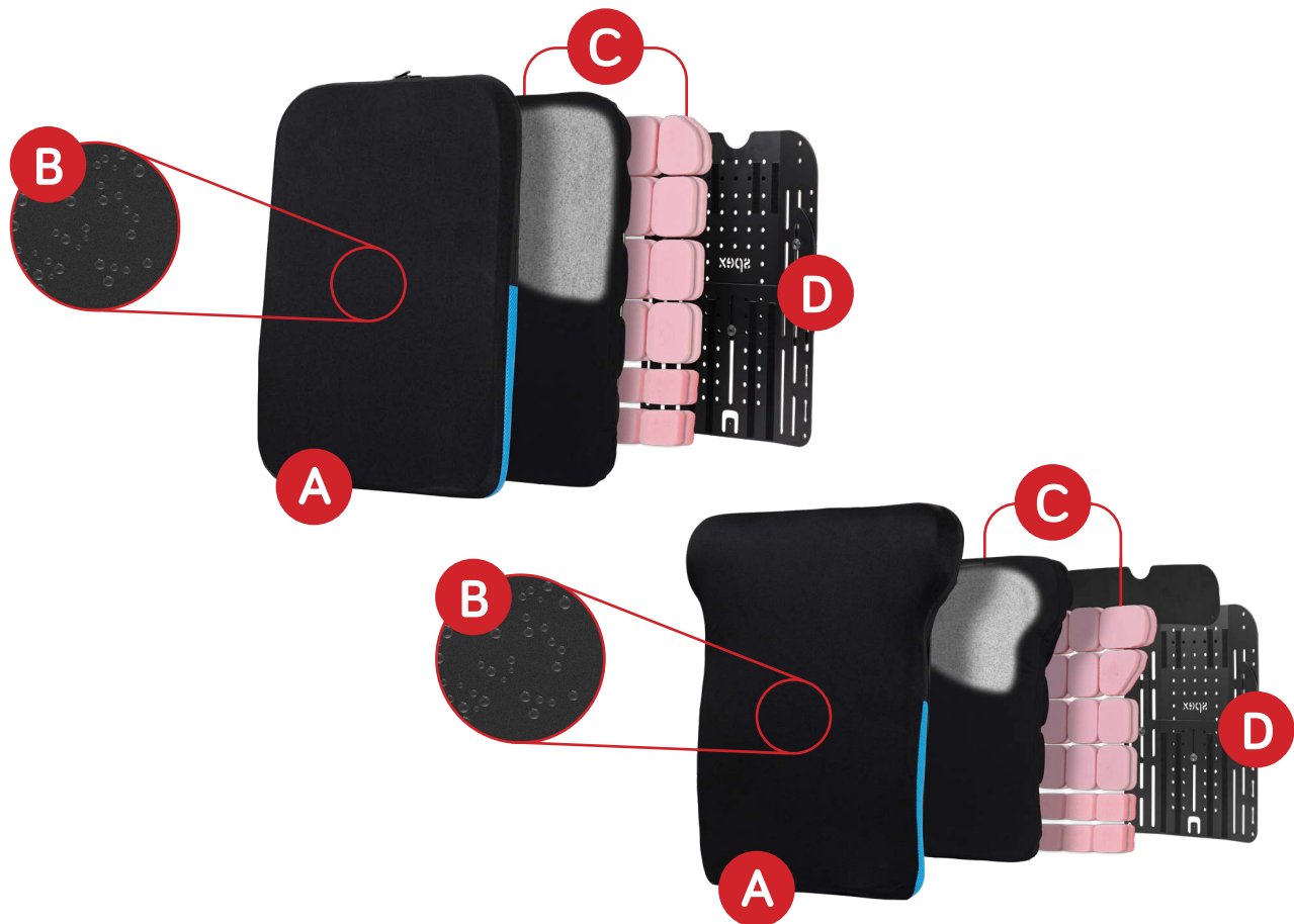
GROWTH-ADJUST SPEX CLASSIC BACK SUPPORT - EXPLODED
